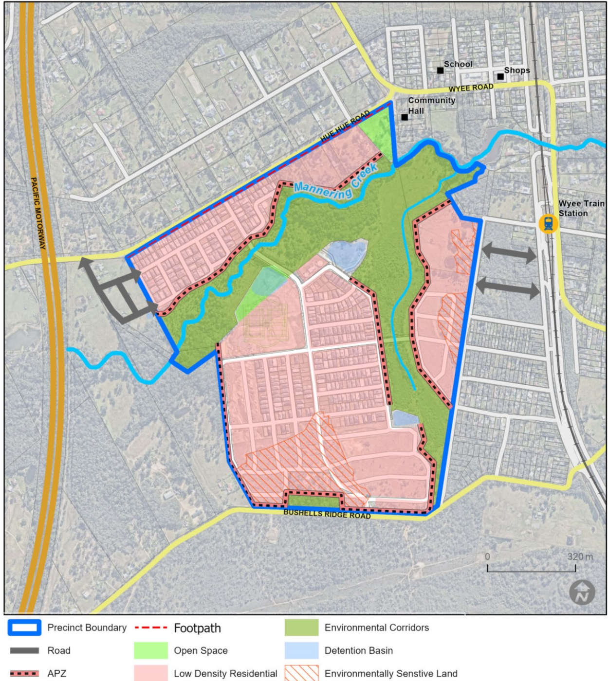
Figure 5 – Precinct A: Subdivision Design and Layout Plan
