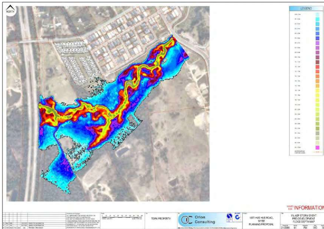
Figure 2 - 1% AEP predevelopment flood extent with original Manning's n values
